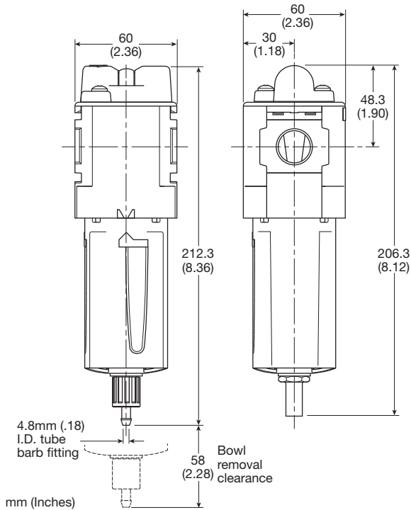
Manual Drain
