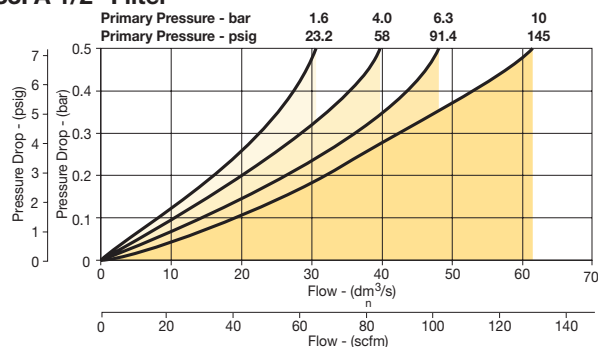
P33FA 1/2" Filter
